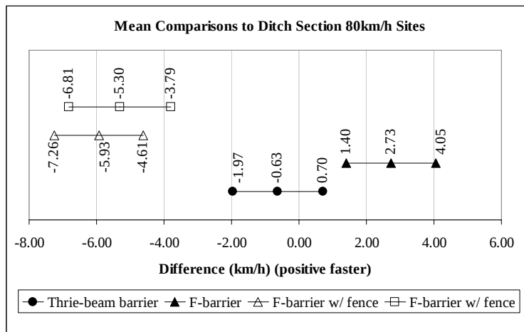
Figure 1: Mean Speed Relative to Ditch Section
