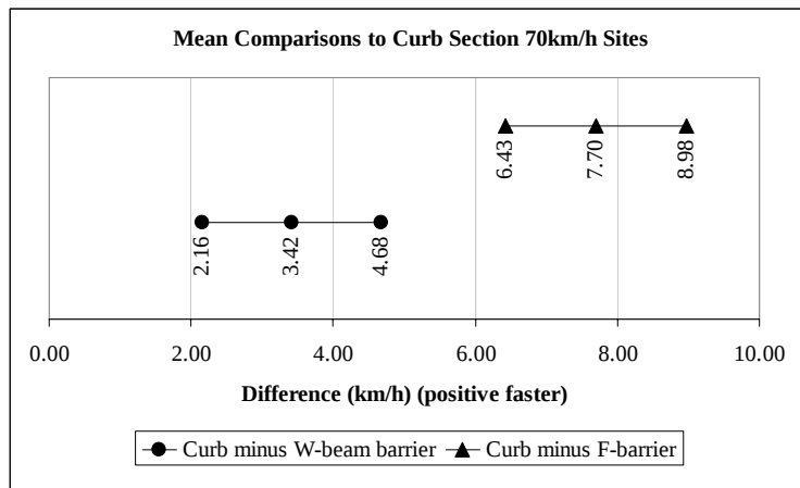
Figure 5: Mean Speed Relative to Raised Curb Section
